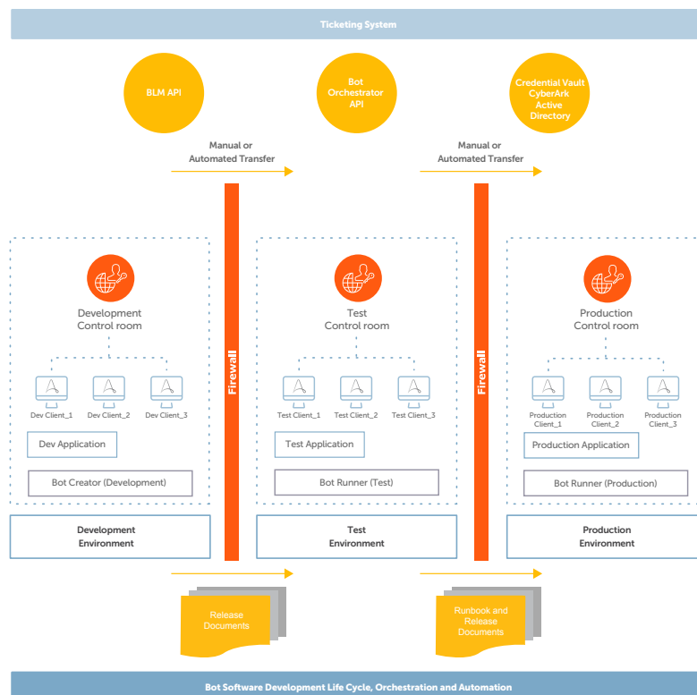
Figure 8: Advanced Deployment Model for full SDLC
